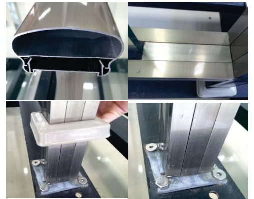
expansion bolt used for concrete floor
